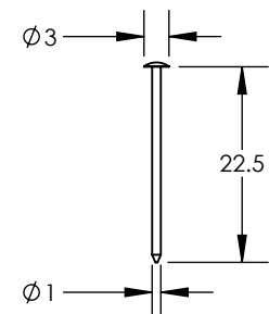
PRETRED APPROVED CONNECTING PIN
